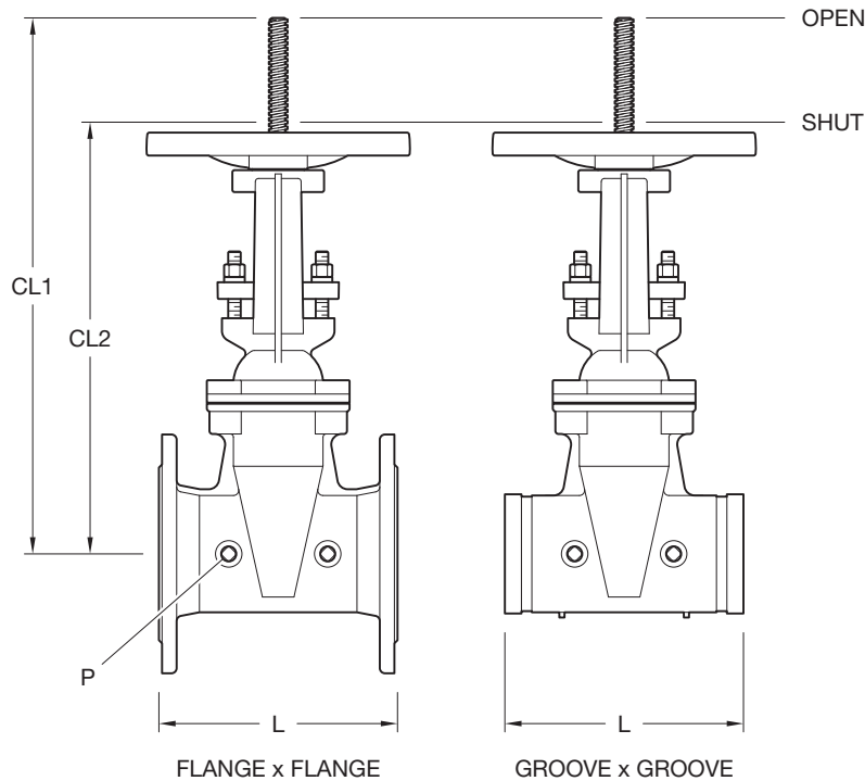
FIGURE 2 OUTSIDE SCREW AND YOKE GATE VALVE DN50 TO DN600 NOMINAL DIMENSIONS
