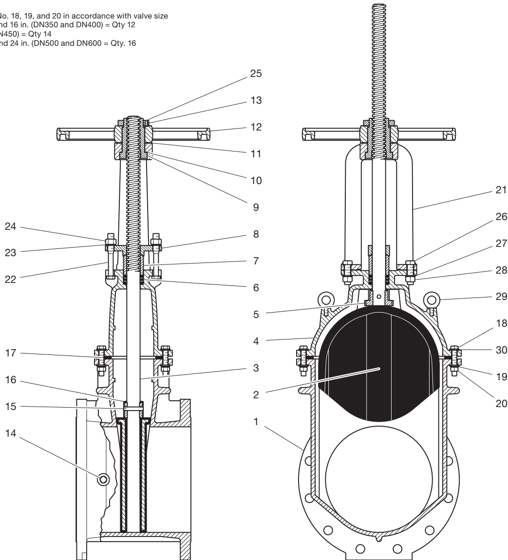
FIGURE 1B OUTSIDE SCREW AND YOKE GATE VALVE 14 IN. TO 24 IN. (DN350 TO DN600) ASSEMBLY
